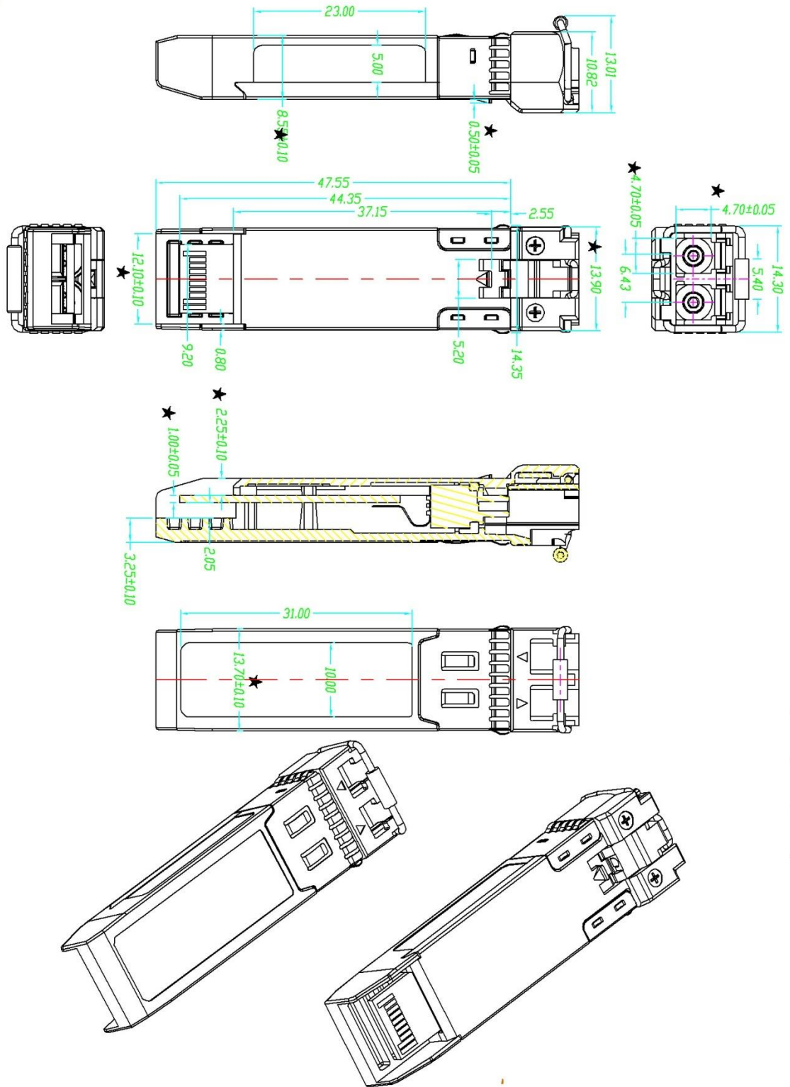
LGP-M85-02D
